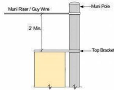
Figure Two: Muni Pole Clearance
