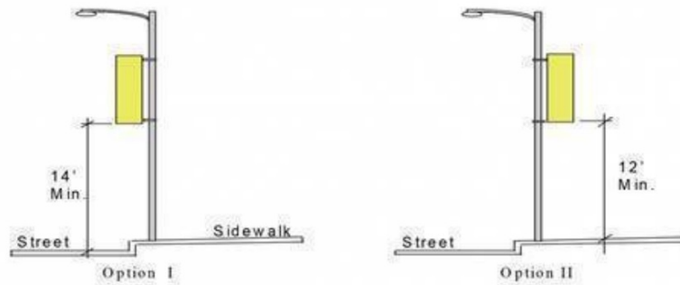
Figure Three: Height Clearances
