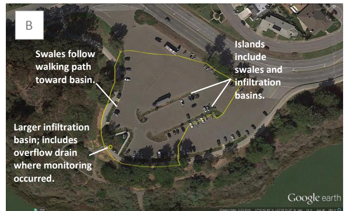
Figure 2. (A) Flows at Sunset Circle were simulated for the pre-construction conditions using SWMM hydrologic modeling software. (B) Post-construction flows were measured in a catchbasin (at yellow circle) located within the large infiltration basin in the southwestern point of the parking lot. Catchment boundary in both aerials shown as yellow outline.
